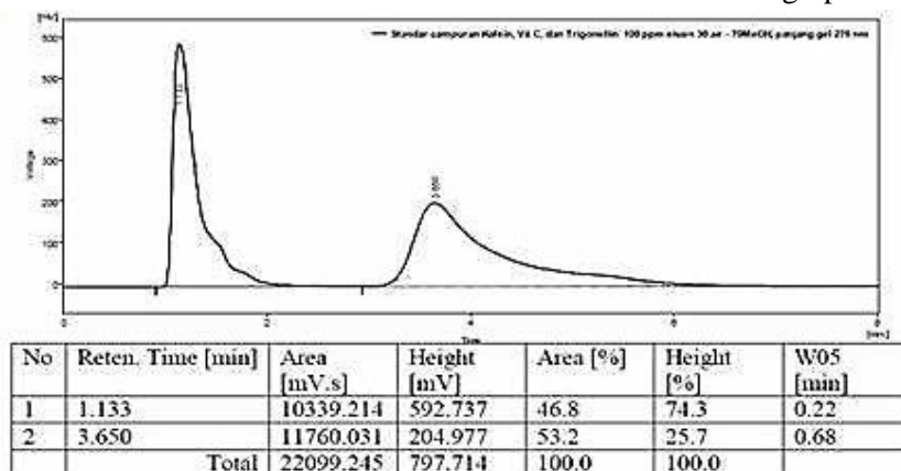
Fig 1. HPLC chromatogram of Caffeine
